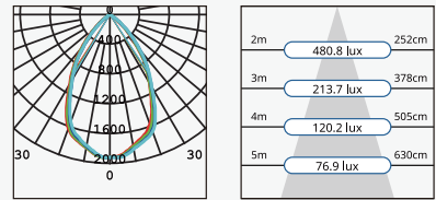
LED20W4000K CFD32A (125-130)
