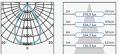
LED35W4000K CFD32A (150-155)
