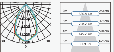
LED24W4000K CFD32A (125-130)
