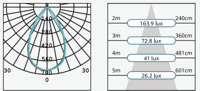
LED7W4000K CFD32A (75-85)
