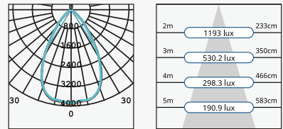
LED40W4000K CFD32A (190-200)
