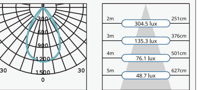
LED12W4000K CFD32A (100-105)
