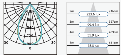
LED9W4000K CFD32A (75-85)
