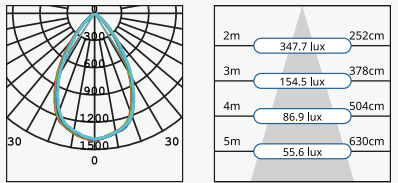
LED15W4000K CFD32A (100-105)
