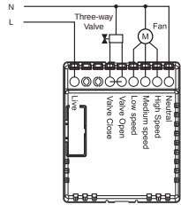
Wiring Diagram of Smart Thermostat (FCU)
