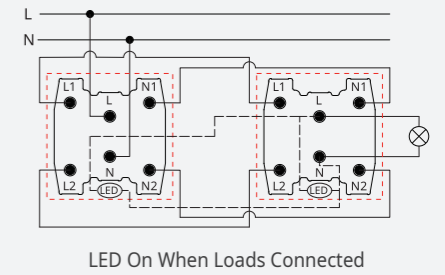
2-way Double Pole Switch
